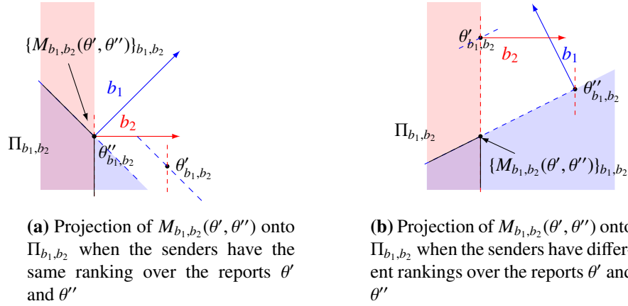
Figure 4: Projection of M_{b_1, b_2}(\theta', \theta'') onto \Pi_{b_1, b_2}
