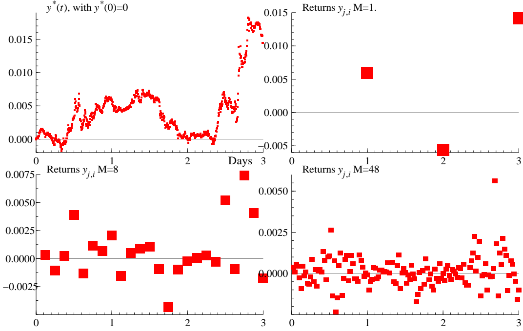
Figure 1: DM/Dollar dataset from the Olsen and Associates database. Top left : raw 5 minute data. Top right : daily returns, M = 1 . Bottom left : 3 hour returns, M = 8 . Bottom right : 30 minute returns, M = 48 .
