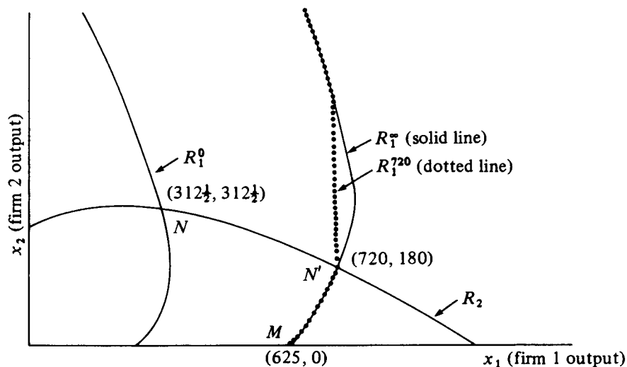
Fig. 1. R_1^0 is 1's reaction curve with no capacity installed (marginal cost = 30). R_1^\infty is 1's reaction curve with infinite capacity (marginal cost = 20). R_1^{720} is 1's reaction curve with 720 units of capacity. R_2 is 2's reaction curve (marginal cost = 30). If 1 installs k_1 \leq 312\frac{1}{2} units of capacity, the equilibrium is at N . If 1 installs 312\frac{1}{2} < k_1 < 720 units of capacity, the equilibrium is along NN' . If 1 installs k_1 \geq 720 units of capacity, the equilibrium is at M .
